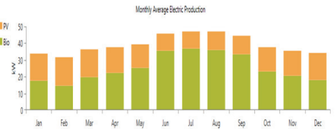
Fig. 7. Energy yield for the proposed system.
