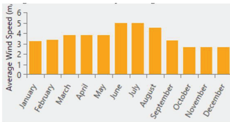
Fig. 3. Normal breeze speed (m/s) for different months.
