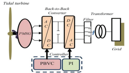
Fig.1.Tidal energy systems configuration based on a PMSG [38]
