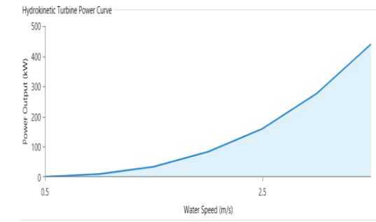
Fig.2. Power Output Curve for the Schottel 54 kW Tidal Turbine
