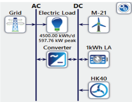
Fig. 13. Proposed system architecture
