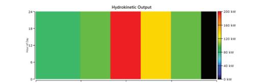
Fig. 17. Hydrokineec Output
