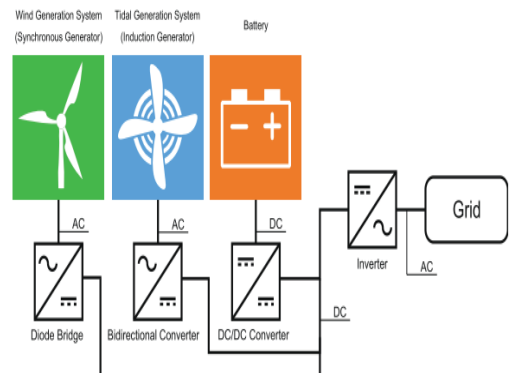
Fig. 12. Conceptual System Schematic of HOTT with Battery [49]
