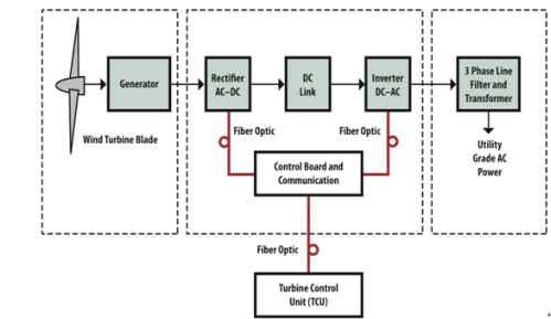
Fig. 3. Block diagram illustrating the components of a wind energy conversion system [39]
