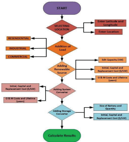
Fig.4. Steps of the model in HOMER
