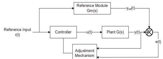
Fig. 2. MRAC system, [7]
