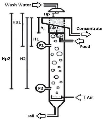
Fig. 1. Pilot Flotation Column, [3]
