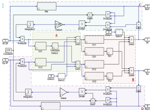
Fig. 4. TwinCAT3 Decoupled MRAC of a Flotation Process
