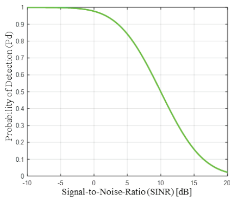
Fig. 6 Probability of Detection
