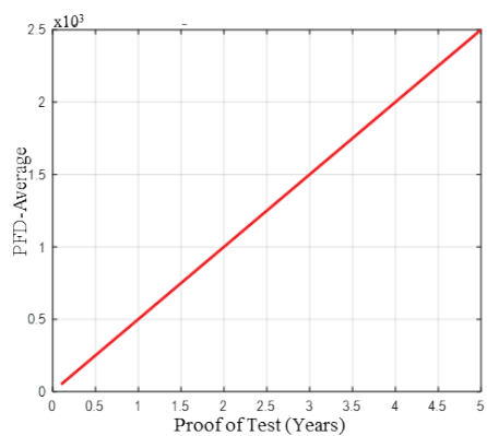
Fig. 4 PFD Average Vs Test Interval for HIPPS in SIL
