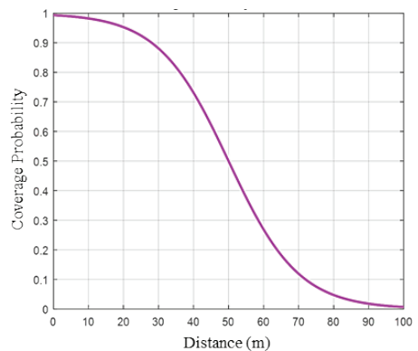
Fig. 8 Coverage Probability vs Distance
