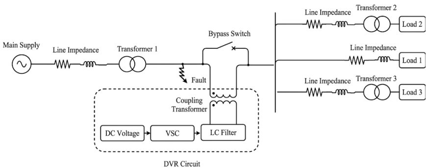
Fig. 1. Single-Line diagram distribution system with DVR
