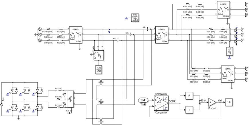
Fig. 2. Simulation circuit with DVR
