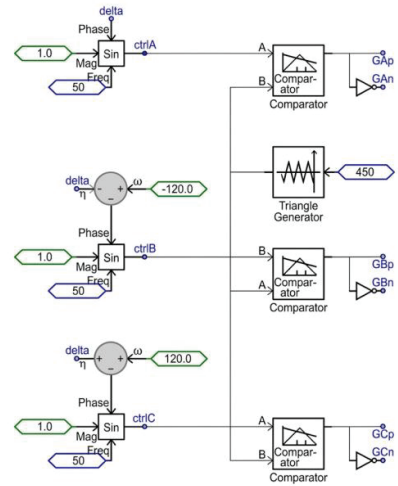
Fig. 4. Configuration pulse width modulation (PWM)
