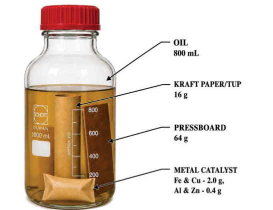
Fig. 2. Close-up view of the materials used in the accelerated thermal ageing experiment.
