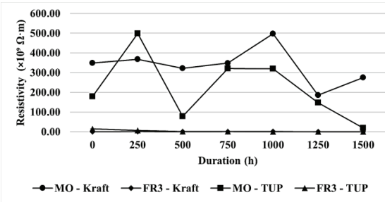
Fig. 6. Volume resistivity (Ω·m) at 90 °C vs. the thermal ageing duration (h). The error bars represent ± standard deviation.
