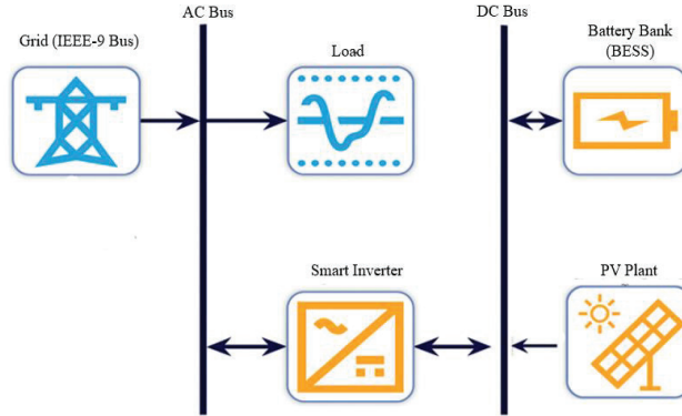
Fig. 1. Schematic of PV-BESS hybrid power system.
