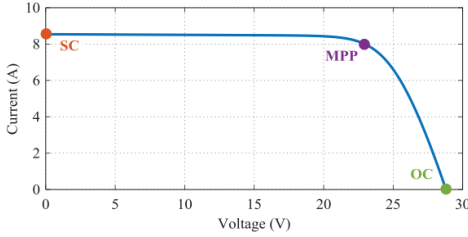
Fig. 4. Photovoltaic I-V curve at STC [16].
