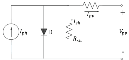
Fig. 3. PV cell single electrical equivalent circuit [16].
