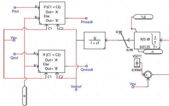
Fig. 5. RTDS adaptive PID-drop voltage controller for PV synchronization in the Grid Following loop.
