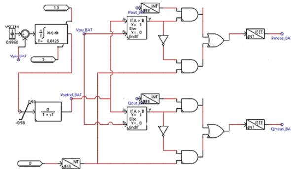
Fig. 6. RTDS PID Controller for BESS integration in Grid Following Power
