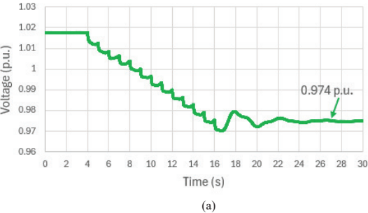
Fig. 10. Comparison of the voltage profile under PV penetration only 10(a) vs. the voltage profile under PV- BESS integration 10 (b) at bus 6.
