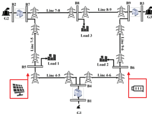
Fig. 2. Modified IEEE-9 bus system with PV-BESS systems[14].
