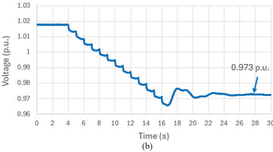
Fig. 11. Comparison of the voltage profile under PV penetration only 10(a) vs. the voltage profile under PV- BESS integration 10 (b) at bus 8.
