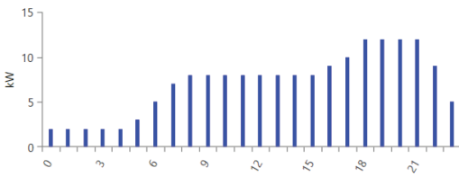
Fig 2. Daily Load Profile
