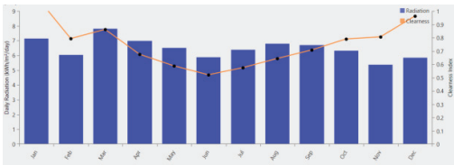
Fig 3. Monthly solar GHI data for FTKE, UTeM
