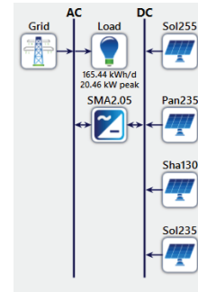
Fig 4. System Architecture
