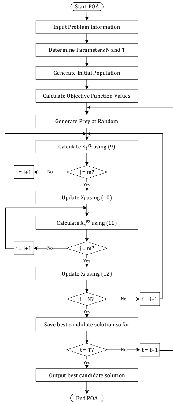
Fig. 2. Implementation Flowchart of POA
