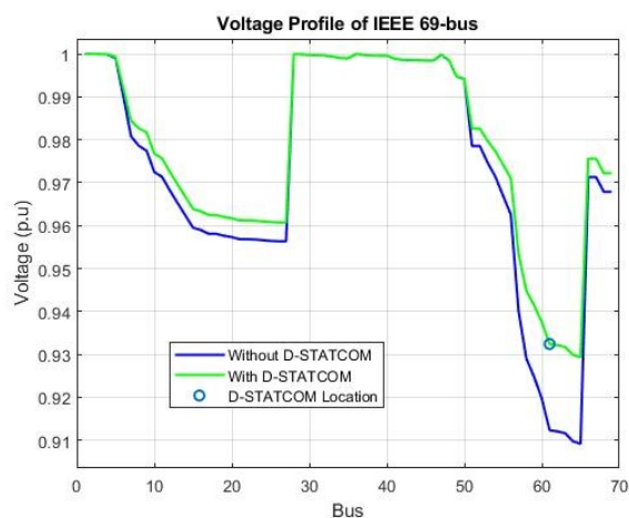
Fig. 6. Voltage profile of IEEE 69-bus system
