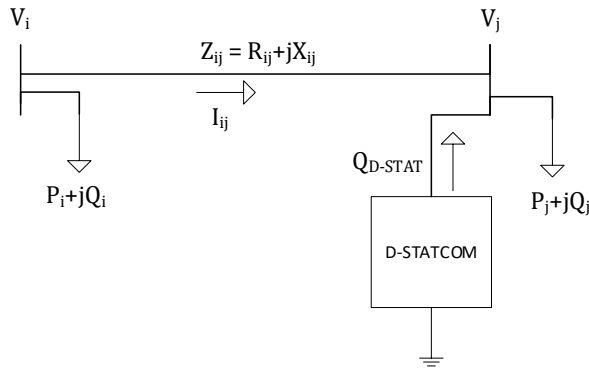
Fig. 1. Illustration of D-STATCOM integrated at bus j
