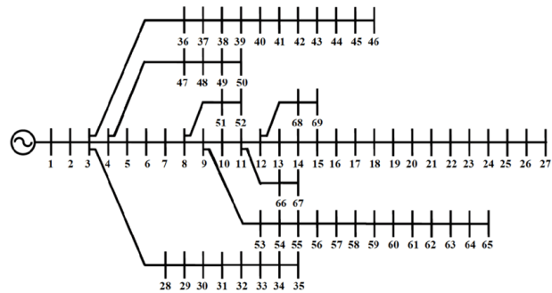
Fig. 5. Single Line Diagram of IEEE 69-bus System
