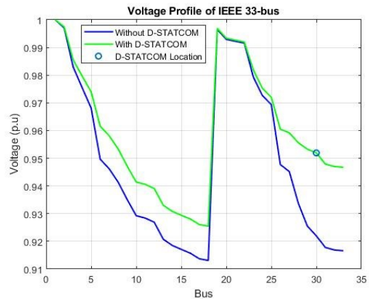
Fig. 4. Voltage Profile of IEEE 33-bus System
