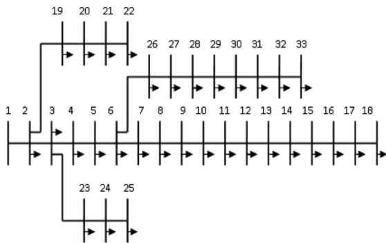
Fig. 3. Single Line Diagram of IEEE 33-bus System
