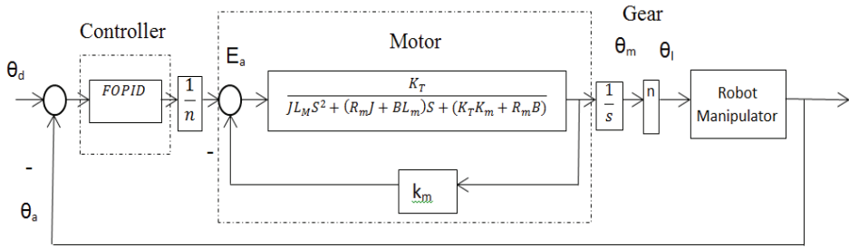
Fig. 4. Robot joint control system
