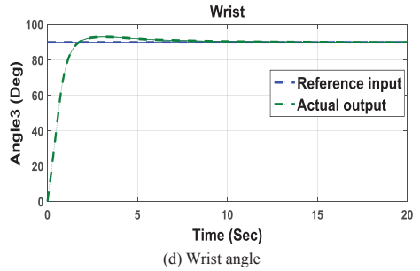
Fig.6. Desired and actual position using PID Controller
