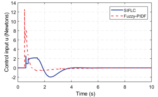
Fig. 10. Control input response
