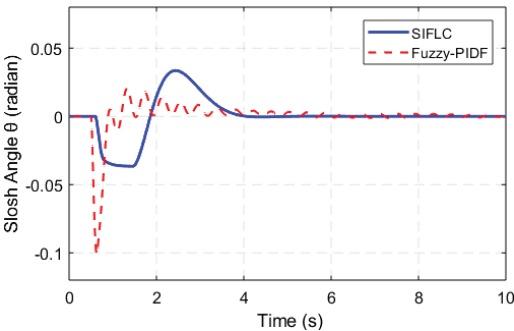
Fig. 8. Slosh angle response
