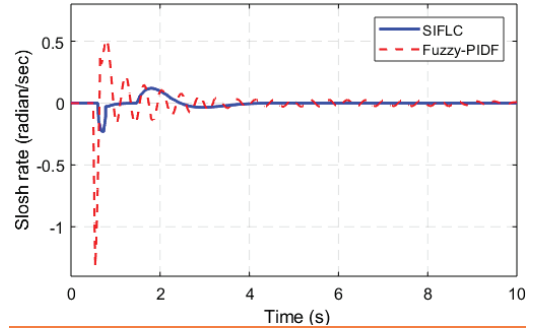
Fig. 9. Slosh rate response
