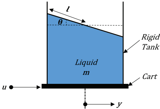
Fig. 1. Liquid slosh motion
