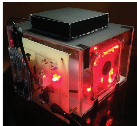
Fig. 12. The system with very high dust level (red LED)
